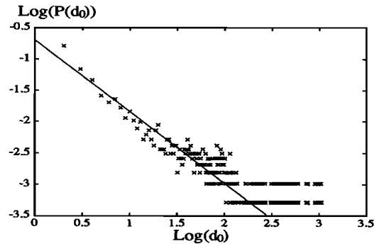
Fig. 3. The return probability histogram P(d_0) in a log-log diagram for one profile. It is the distribution of intercept length of the profile with horizontal lines starting at each point of the profile. A best fit is shown as a straight line of slope -1.14 (giving \zeta = 0.86 ).
