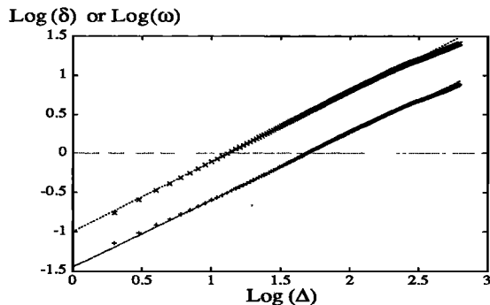
Fig. 2. The difference between the maximum and the minimum height \delta ( \times ) and the standard deviation w = \sqrt{\langle h^2 \rangle - \langle h \rangle^2} ( + ) on bands of width \Delta are shown in a log-log diagram. The two straight lines are best fits of slopes 0.89 ( \cdots ) and 0.85 ( - - ) respectively.
