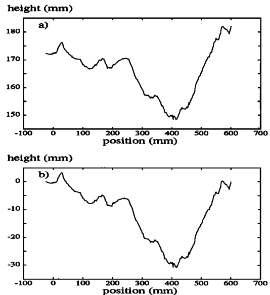
Fig. 1. (a) is one of the 6 raw profiles taken over the granitic fault surface. The height is plotted as a function of position. (b) is the filtered profile obtained by subtracting the drift between the first point and the last one.
