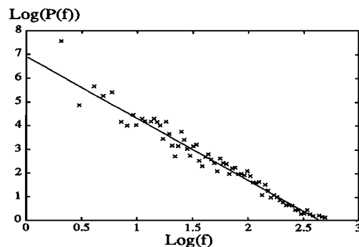
Fig. 4. The power spectrum P(f) of the profile as a function of the frequency f in a log-log diagram. A linear regression of slope 2.60 is shown. The corresponding value of the roughness exponent is 0.80.
