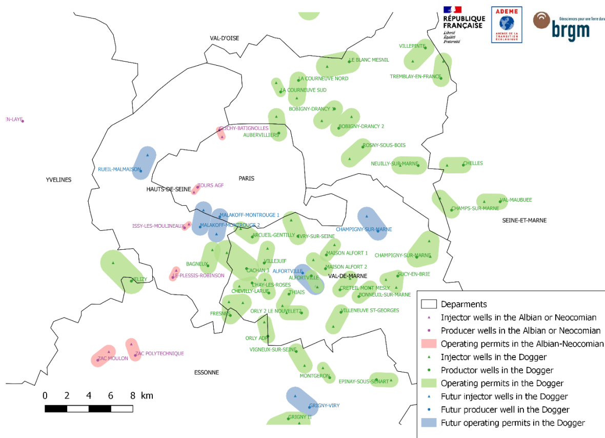
Figure 1: Localisation of the geothermal doublets tapping the Albian or Neocomian sands (pink) or the Dogger Limestones (green and blue) in Paris area
