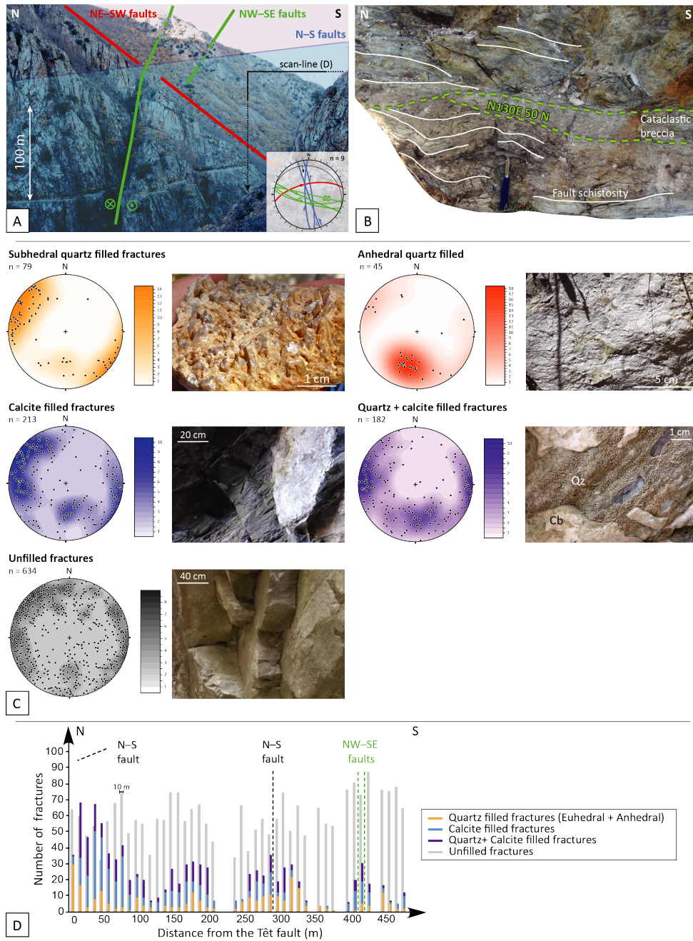
FIGURE 8: Faults and fractures inside the Carança canyon (see location Figure 6). A) Landscape view of the Carança canyon, and stereograms of the faults. View since N042.51470;E002.22482, B) Outcrop of a NW-SE ductile fault reactivated as brittle (N042.51799;022.22368, C) Stereograms and pictures of the different types of fracture filling, D) Scan-line of fractures amount each 10 m as a function of the filling. The scan-line starts at the Têt fault, in the footwall, at the entrance of the canyon (N042.52166;E002.22173). No corrections (e.g., Terzaghi) have been applied.
