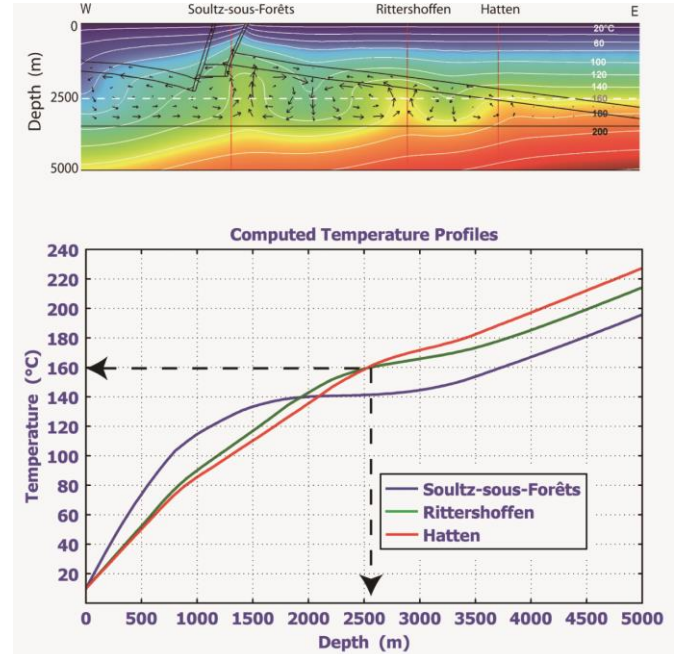
Figure 2 – Numerical simulation of hydrothermal convection in the Upper Rhine Graben. The 2D west-east section crosses the Soultz-sous-Forêts thermal anomaly. Permeability values are chosen to reproduce the measured temperature profile. For the two other anomalies (Rittershoffen and Hatten), higher temperatures at a depth of 2000-2500m are predicted.
