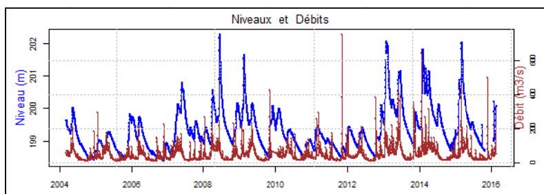
Figure 3 – Discharge in the Gave d'Oloron (Q7002910) and water table levels measured by piezometer 10295X0032
