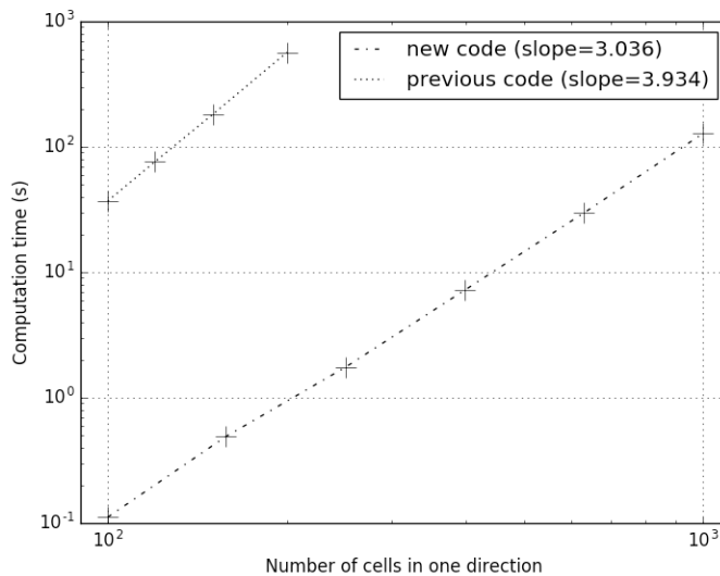
Figure 3: Computation time for different grid sizes and for the new code (dashed line) and our previous code (dotted line). All grids are n \times n , n varying from 10^2 to 10^3 ; the total number of cells, n^2 , varies from 10^4 to 10^6 . The slope of each curve is estimated through linear regression.
