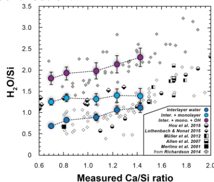
Figure 1. Plots of \text{H}_2\text{O/Si} against \text{Ca/Si} with the gray diamonds are adapted from 5. The blue circles are for interlayer water, the light blue ones for interlayer water and a single adsorbed monolayer and the purple ones are with the contribution of hydroxyls from this work.
