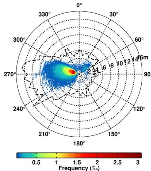
Figure 3. Polar representation of waves' characteristics for the point 'Brittany_09'.
