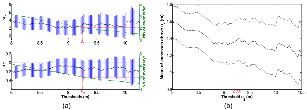
Figure 4. (a) Stability of modified scale and shape parameters for the GPD. The vertical blue bars represent the 95% confidence intervals; (b) Linearity of the mean residual life plot. The dashed lines represent the bounds of the 95% confidence interval.
