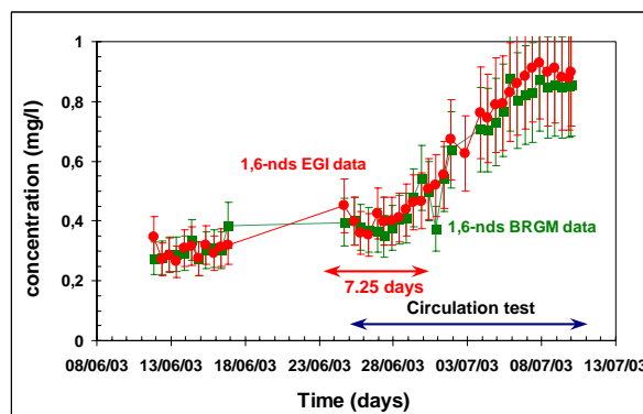
Figure 8 - Geochemical monitoring of the fluid discharged from the well GPK-2 (from 11/06 to 9/07/2003): Analytical results of the 1,6-nds tracer injected into GPK-3 in 2003.
