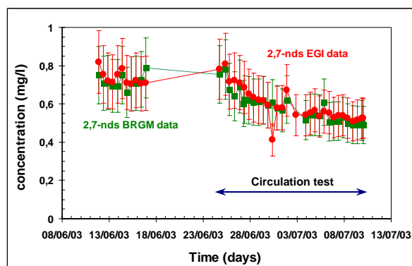
Figure 7 - Geochemical monitoring of the fluid discharged from the well GPK-2 (from 11/06 to 9/07/2003): Analytical results of the 2,7-nds tracer injected into GPK-2 in 2003.
