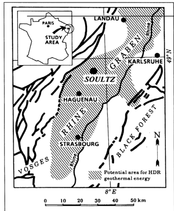
Figure 1 - Location map of the Rhine Graben and Soultz-sous-Forêts.
