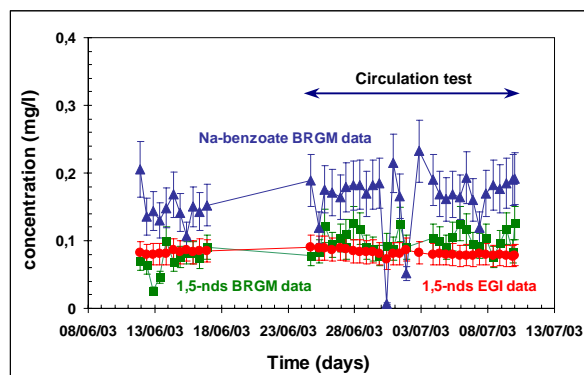
Figure 6 - Geochemical monitoring of the fluid discharged from the well GPK-2 (from 11/06 to 9/07/2003): Analytical results of the organic tracers injected into GPK-2 in 2000 (Na-benzoate and 1,5-nds).
