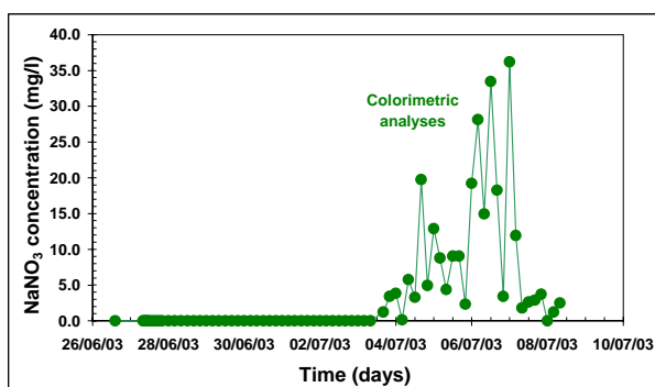
Figure 5 - Geochemical monitoring of the fluid discharged from the well GPK-2 (from 26/06 to 9/07/2003): Analytical results of the NaNO 3 tracer obtained using the colorimetric technique on site.
