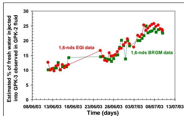
Figure 10 - Estimation of the proportions of the fluid injected into GPK-3 in 2003, relative to the total mass of fluid discharged from the well GPK-2 (from 11/06 to 9/07/2003), using the concentrations of 1,6-nds.
