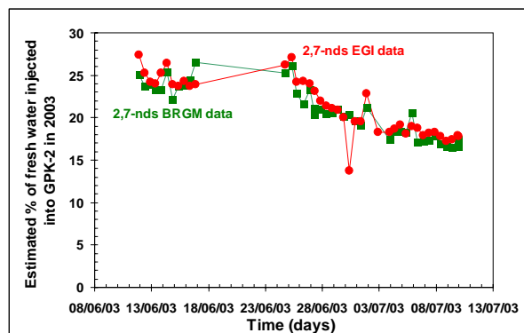
Figure 9 - Estimation of the proportions of the fresh water injected into GPK-2 in 2003, relative to the total mass of fluid discharged from this well (from 11/06 to 9/07/2003), using the concentrations of 2,7-nds.
