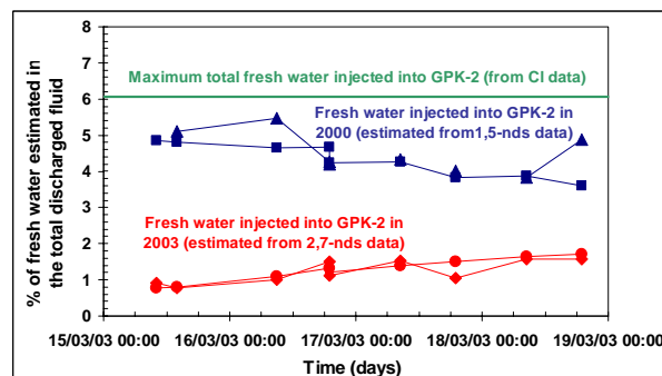
Figure 4 - Estimation of the proportions of fresh water injected into GPK-2 in 2000 and 2003, relative to the total mass of fluid discharged from the well GPK-3 (March 2003), using the concentrations of Cl and organic tracers (1,5-nds and 2,7-nds).
