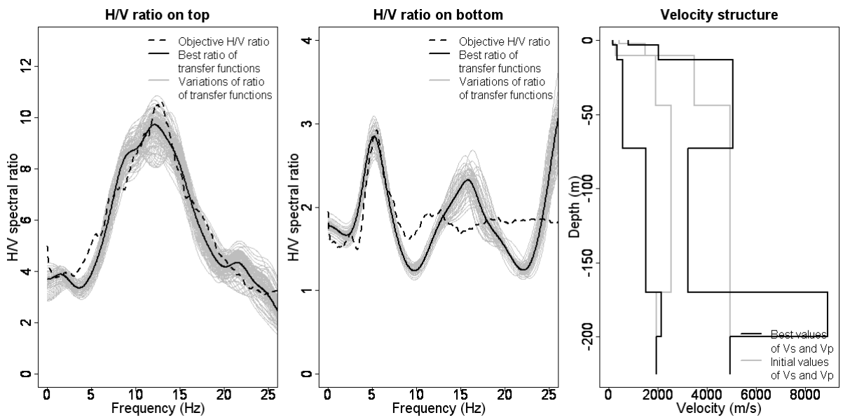
Figure 3.2. Result of inversion for station FKSH09
