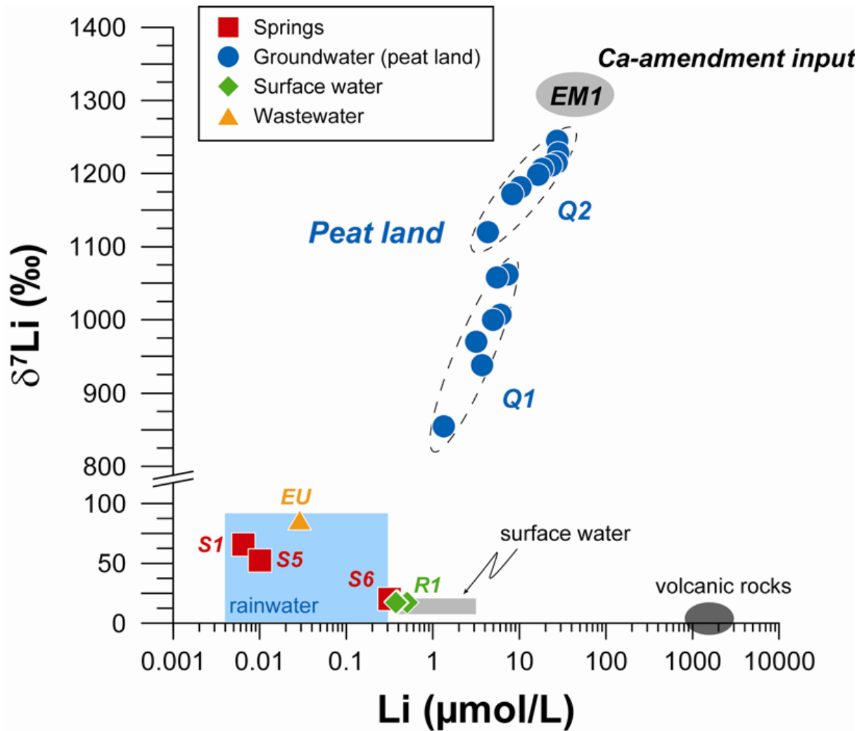
631 632 Figure 5. Plot of \delta^7\text{Li} vs. Li concentration ( \mu\text{mol. L}^{-1} ) for groundwater from the peatland (Q1 633 and -Q2), spring water S1 and S5 located on the hillslope on the western side and S6 634 (emerging close to the outlet of the area), wastewater EU and surface water R1 in the 635 Narces de la Sauvetat peatland. Rainwater, volcanic rocks and surface water from the 636 Massif Central are also indicated (see text). The end-member EM1 corresponds to the 637 carbonate amendment input. Its location on the graph is assumed to represent the required 638 lithium content-Li isotope ratios to take all data into account.
