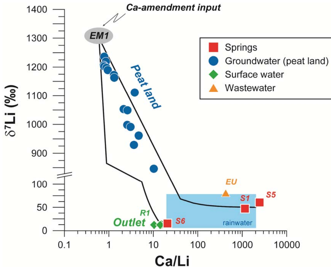
648 649 Figure 7. Plot of \delta^7\text{Li} vs. Ca/Li ratios for groundwater from the peatland (Q1 and -Q2), spring 650 water S1 and S5 located on the hillslope on the western side and S6 (emerging close to the 651 outlet of the area), wastewater EU and surface water R1 in the Narces de la Sauvetat 652 peatland. The end-member EM1 corresponds to the carbonate amendment input. Its 653 location on the graph is assumed to represent the required Ca/Li and Li isotope ratios to 654 take all data into account. Two different mixing lines can then be calculated between the 655 end-member EM1, representing the application of carbonate amendment, the S6 spring 656 water and other spring waters (see text).
