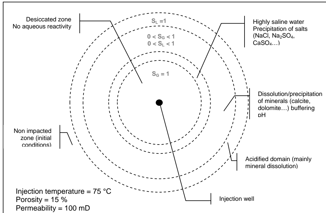
Figure 14: Typical radii of processes occurring in the near-well region after CO 2 injection in a saline aquifer (Azaroual et al. 2007 and Gaus et al. 2008)
