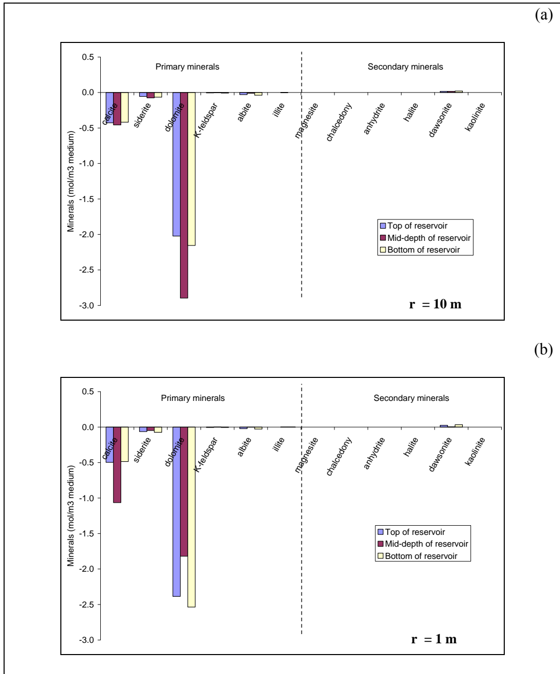
Figure 6: Results obtained from Scenario 1B - Variation in mineral concentrations around the injection well after a 300-day period of supercritical CO 2 injection (flow rate = 1 kg s -1 and T = 40 °C): (a) 10 m; (b) 1 m. Negative values correspond to dissolution and positive values to precipitation.
