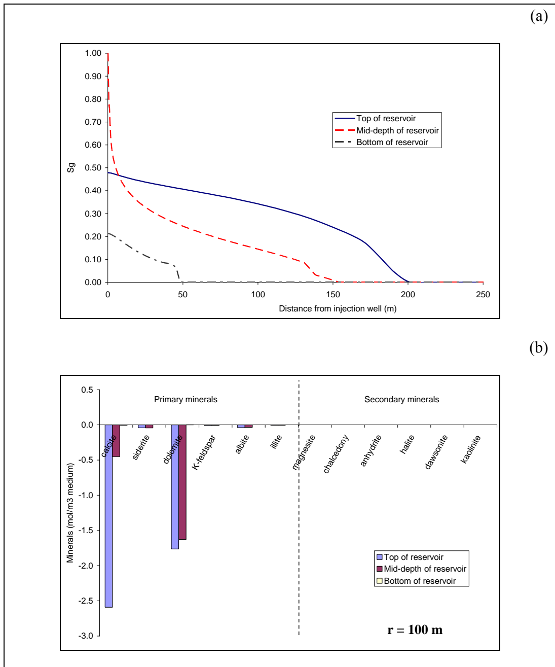
Figure 3: Results obtained with Scenario 1A: (a) Spatial evolution of gas saturation within the reservoir after a 300-day period of supercritical CO 2 injection at 1 kg s -1 and 75 °C; (b) Quantity of dissolved minerals (mostly carbonates) 100 m from the injection well.
