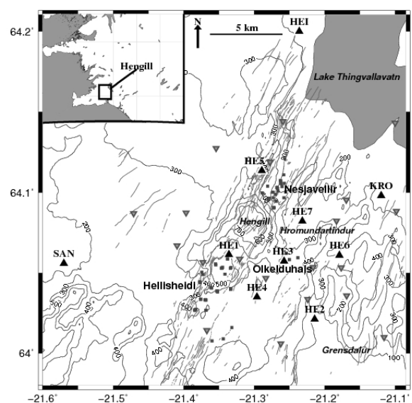
Figure 2 – Topographic map of Hengill Volcano, Iceland, with the location of the broadband seismological stations (HE1, HE2, HE3, HE4, HE5, HE6, HE7) and SIL network stations (KRO, SAN, HEI). Small gray squares are locations of geothermal wells; they are grouped in three areas (Nesjavellir, Hellisheidi and Olkelduhals). The three main volcanic centers are indicated in italics (Hengill, Hrómundartindur and Grændalur). Grey lines represent fissure swarms at surface. Inset shows the location of Hengill volcano in Iceland.
