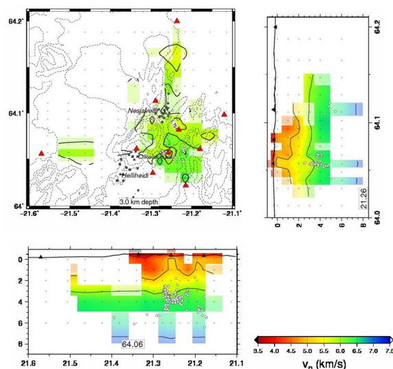
Figure 3 – v_p velocity model from the joint inversion of hypocenters and velocity model for two vertical slices and an horizontal slice at 3 km depth.
